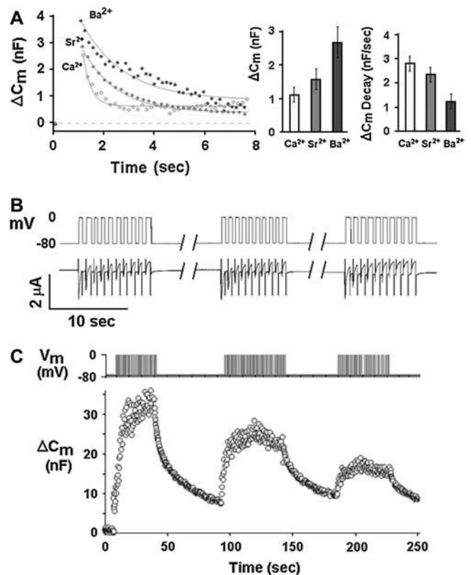
FIGURE 5 Differential effects of Ca 2+ , Sr 2+ , or Ba 2+ on depolarization-induced C_m changes, and vesicle depletion by repetitive stimulation (A) Differential effects of Ca 2+ , Sr 2+ , or Ba 2+ on depolarization-induced exocytosis. Oocytes expressing Ca v 1.2, syntaxin 1A, syt-1, and SNAP-25 (excitosome). (Left panel) Original traces showing time course of C_m upon depolarization, fitted by simple exponentials; (middle panel) instantaneous depolarization-induced \Delta C_m increase in Ca 2+ , Sr 2+ , and Ba 2+ (mean \pm SE, n = 10 , each); and (right panel) rate of compensatory C_m decrease (mean \pm SE, n = 10 , each). As compared to Ca 2+ , the instantaneous C_m increase was greater in Ba 2+ (middle panel), and the compensatory C_m decrease was slower (right panel). In Sr 2+ , the respective values were between those of Ca 2+ and Ba 2+ . (B) Current amplitude during repeated trains of membrane depolarization. Oocytes were depolarized by three trains composed of 10 depolarizations from -80 to 0 mV 1 s each (upper panel). Depolarization-induced inward current inactivated during trains whereas no run-down of current amplitude was observed from one train to the other (lower panel). (C) Exhaustibility of depolarization-induced capacitance changes. Repeated depolarization pulses from -80 mV to 0 mV for 1 s each (upper trace) and the associated C_m changes (lower trace). Data are consistent with depletion and only partial replenishing of a pool of releasable vesicles.
