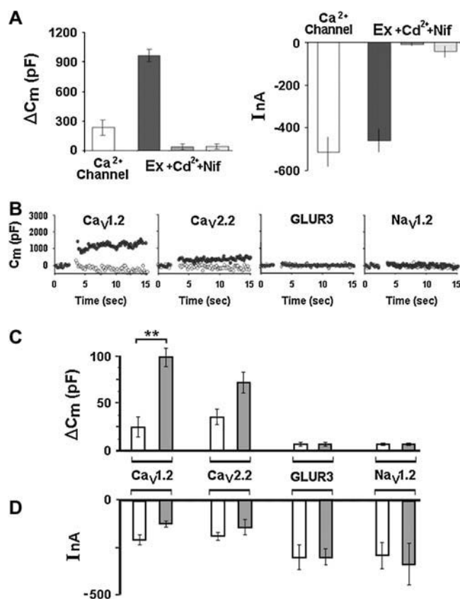
FIGURE 6 Dissecting out the role of the \text{Ca}^{2+} channel in reconstituted depolarization-induced exocytosis. (A) Effect of \text{Ca}^{2+} channel inhibitors on reconstituted depolarization-induced exocytosis. Oocytes were expressing either the Lc-type \text{Ca}^{2+} channel alone (leftmost bar), or together with the synaptic proteins syntaxin 1A (sx1A), synaptotagmin I (syt I), and SNAP-25 (other three bars). Depolarization-induced changes of capacitance ( \Delta C_m ) and current amplitude ( I ) in 5 mM \text{Ba}^{2+} . The effects of the \text{Ca}^{2+} channel blockers \text{Cd}^{2+} (200 \mu\text{M} ) and nifedipine (10 \mu\text{M} ) show that depolarization-induced exocytosis absolutely requires the presence and functionality of a voltage-gated \text{Ca}^{2+} channel. (B) Effect of channel type on depolarization-induced C_m changes. Time course of C_m in oocytes expressing various voltage-gated channels (L-, N-type \text{Ca}^{2+} channels, GluR3 receptor, or brain-type II \text{Na}^{+} channel; see Methods) without (open circles) or with SNAP-25, syntaxin 1A, and synaptotagmin 1 (solid circles); bath containing 5 mM \text{Ba}^{2+} (with \text{Ca}^{2+} channels and GluR3) or 50 mM \text{Na}^{+} (with \text{Na}^{+} channel). Depolarization from -80 mV to 0 mV for 2 \times 500 ms. (C) Effect of channel type on size of depolarization-induced C_m increase. Same protocol as in (A) (open bars) channel only; (solid bars) channel plus SNAP-25, syntaxin 1A, and synaptotagmin 1. Mean \pm SD from 10 oocytes, each. \text{Ca}_v1.2 versus \text{Ca}_v1.2 + synaptic proteins (**), P < 0.0015 ; \text{Ca}_v2.2 versus \text{Ca}_v2.2 + synaptic proteins P^* < 0.1 in Student's t -test. (D) Effect of channel type on depolarization-induced current changes. Same protocol as in A and B.
